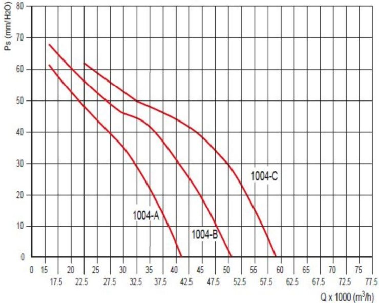
DUCT-M-HT 1000 - 4 poles
