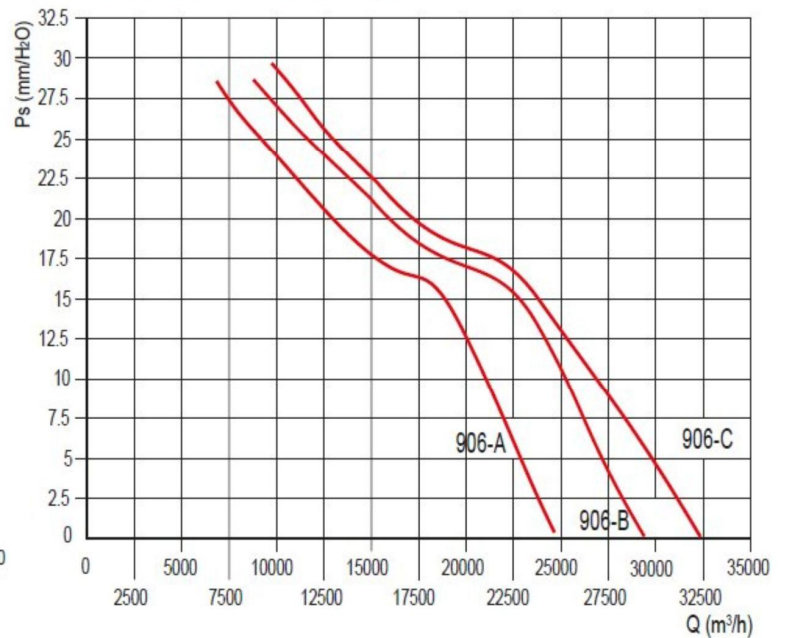
DUCT-M-HT 1000 - 6 poles
