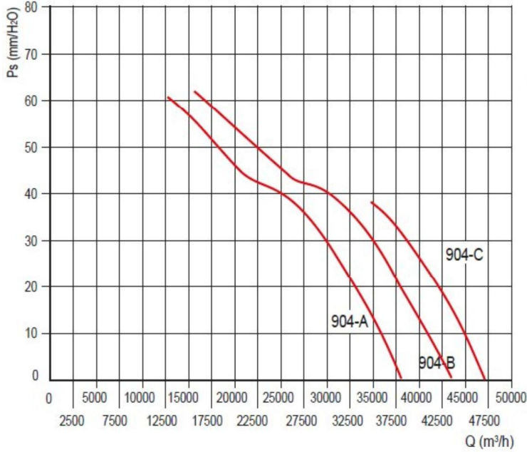
DUCT-M-HT 1000 - 4 poles
