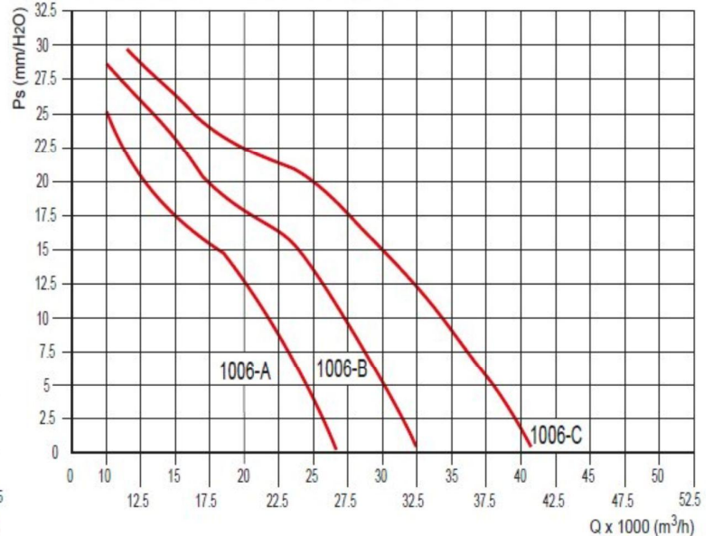
DUCT-M-HT 1000 - 6 poles
