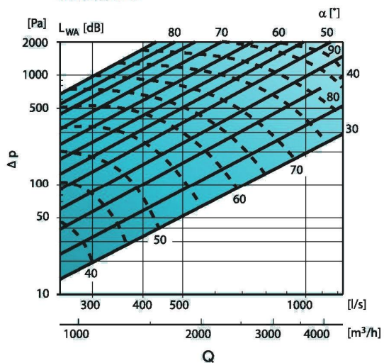
AKH Ø315
