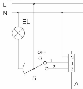
Diagram 4
