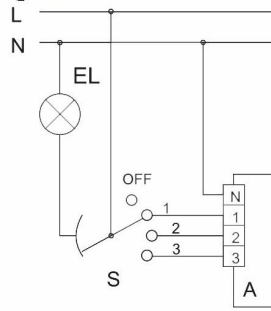
Diagram 4
